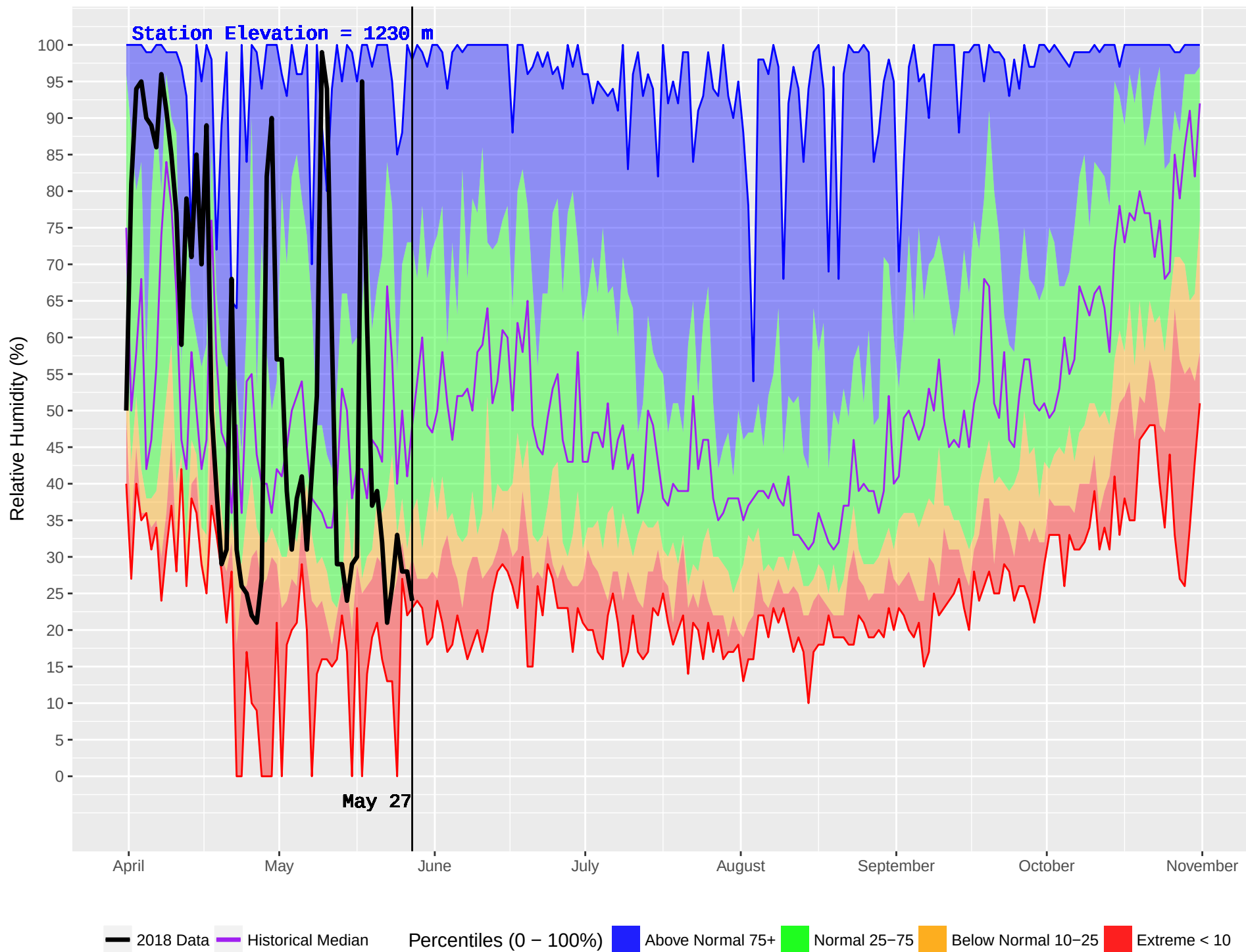
SLOCAN (406) : Historical (1992–2016) and Current (2018) Noon Relative Humidity
