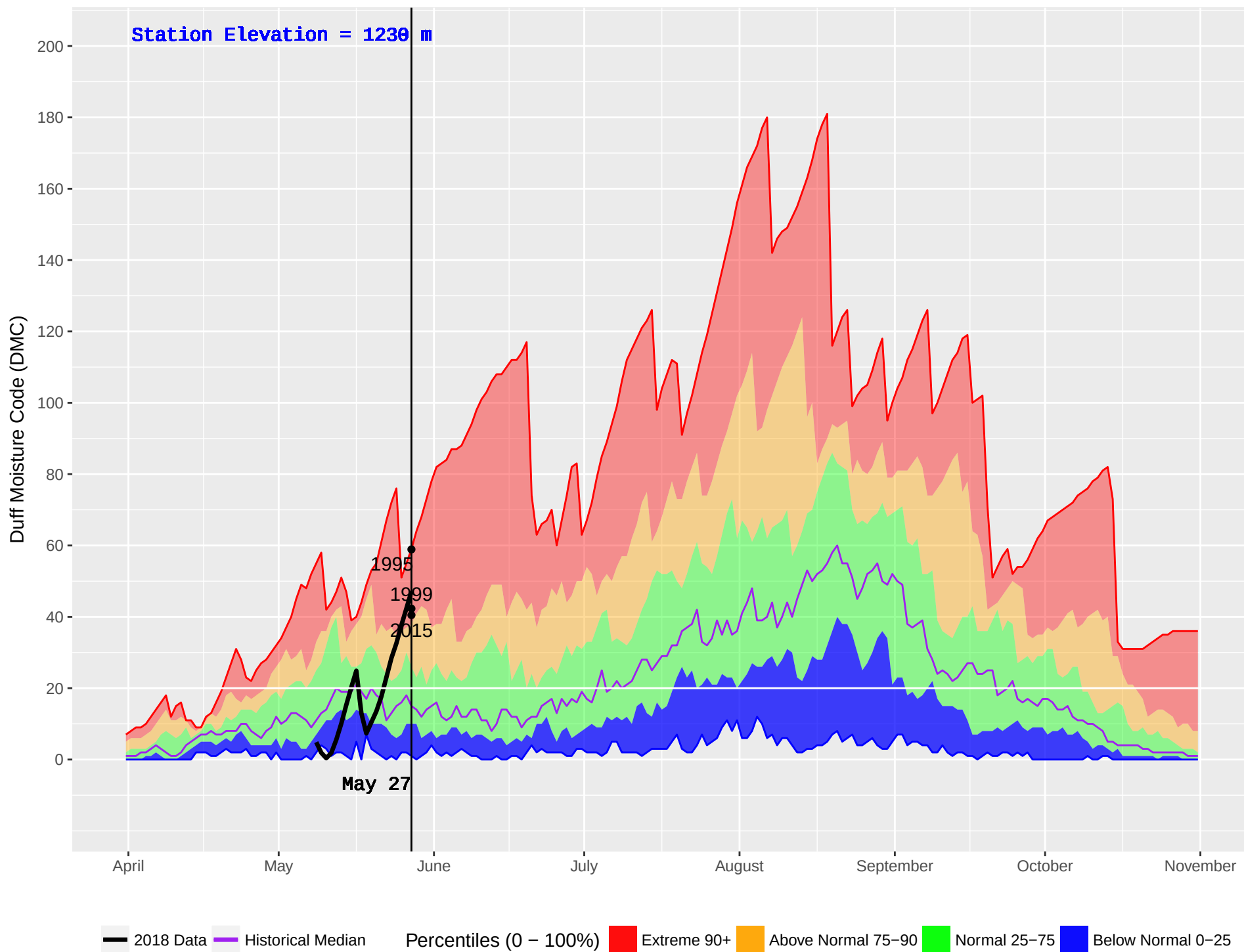
SLOCAN (406) : Historical (1992–2016) and Current (2018) Noon Duff Moisture Code (DMC)
