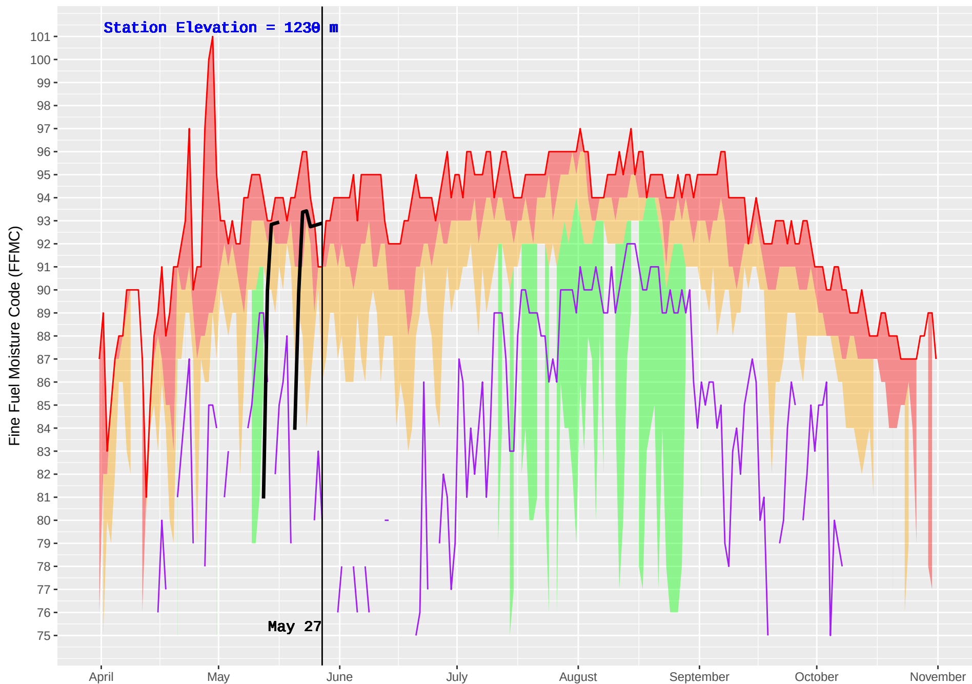
SLOCAN (406) : Historical (1992–2016) and Current (2018) Noon Fine Fuel Moisture Code (FFMC)
