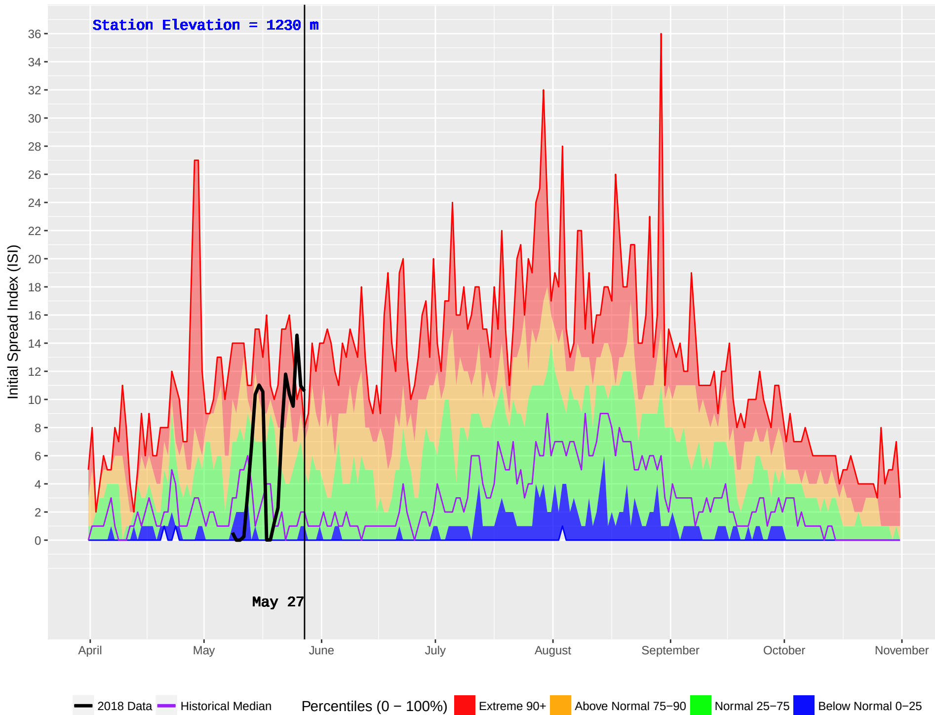
SLOCAN (406) : Historical (1992–2016) and Current (2018) Noon Initial Spread Index (ISI)
